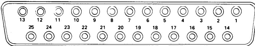
Figure 3: Numbering on a female RS-232 connector. (see Model 100 manual)
