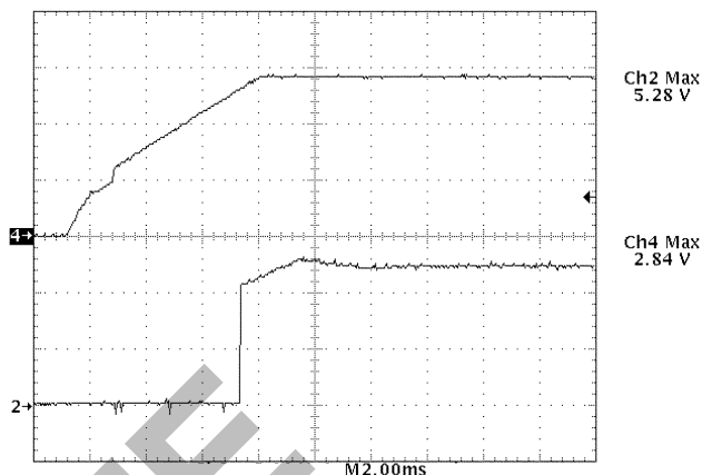
Trace 2– PWRGD (2.0 V/div.) Trace 4– V<sub>OUT</sub> (1.0 V/div.)
