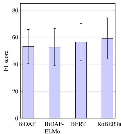
(b) F1 mean and standard deviation over 4 human voices. For details and score breakdown by speaker, see Appendix D.
