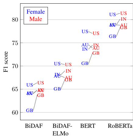
(a) F1 scores for TTS voices over 4 accent and 2 gender settings. Lines connect the results for different gender but same accent and model.
