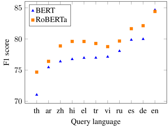
Figure 2: Effect of the input language on the QA system performance in an MT pipeline. Automatically translating non-English queries to English decreases performance for all source languages, and the decrease is especially noticeable for lower-resource languages.
